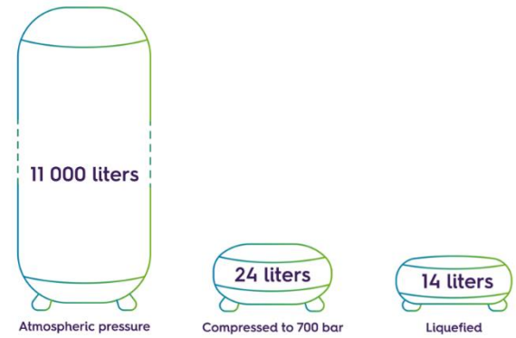
Figure 2. Storage volume for 1kg of hydrogen in different state [7]
