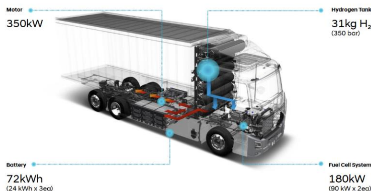
Figure 23. XCIENT Fuel Cell Truck [79]
