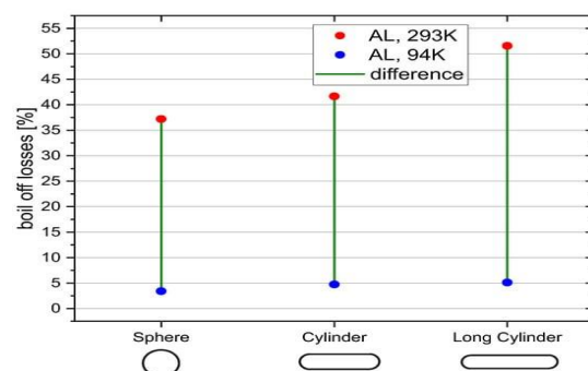
Figure 4b. Boil off rates by storage shape [11]
