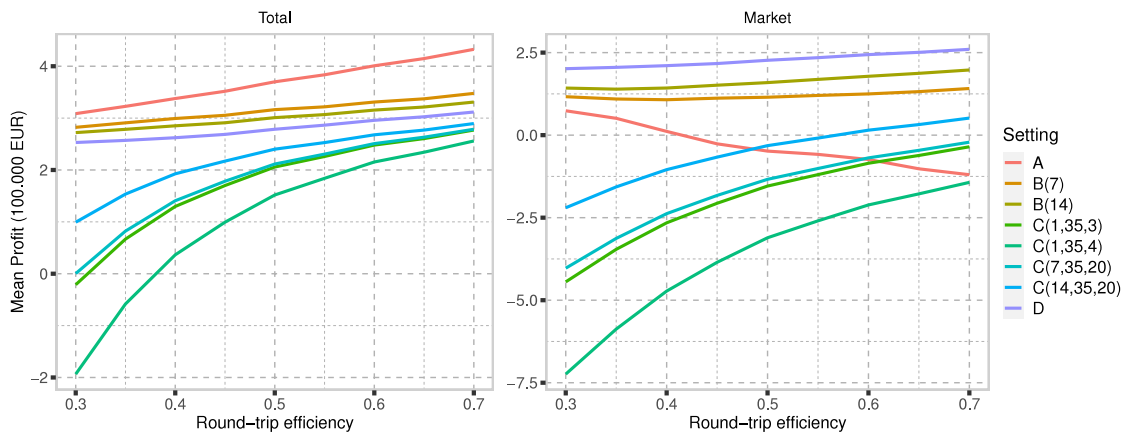
Fig. 6. Impact of round-trip efficiency on the total expected rewards for the settings A – D.
