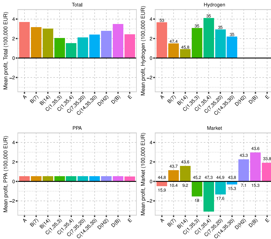
Fig. 2. Total profit, hydrogen market profit, PPA profit and electricity market profit for base case.
