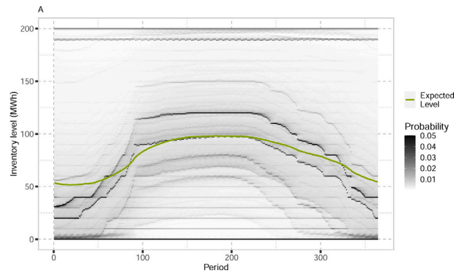
Fig. 3. Heatmap of inventory level in tank over time, for setting A.
