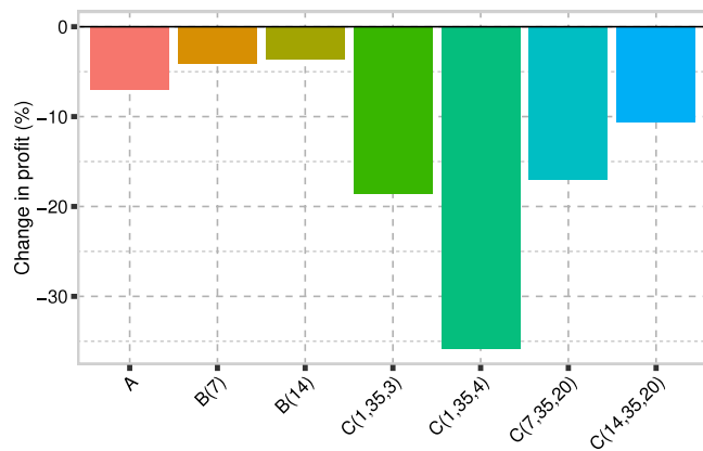
Fig. 7. Relative change in profit of each setting in case \alpha = 0.10 compared to \alpha = 0.0 .
