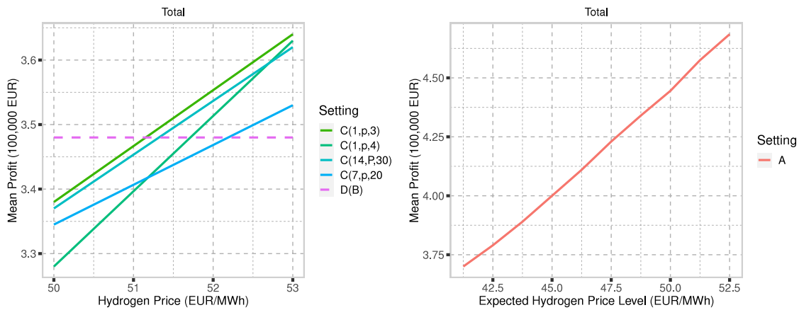
Fig. 4. Impact of higher fixed hydrogen price on profit of settings with hydrogen offtake agreements, and impact of higher expected hydrogen market price (right) for setting A.
